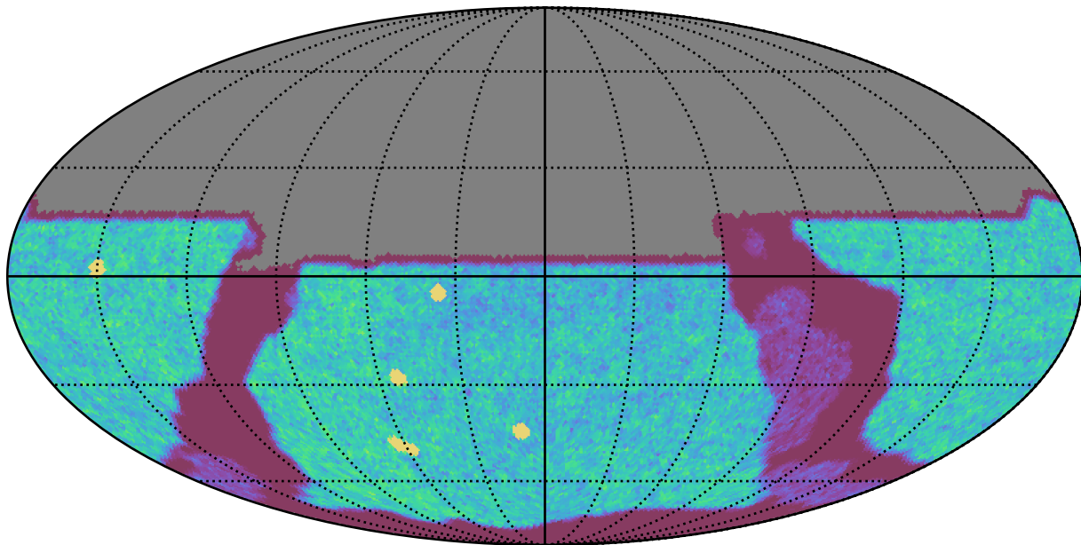
ddf_half_v3.4_10yrs All sky u band: NVisits
