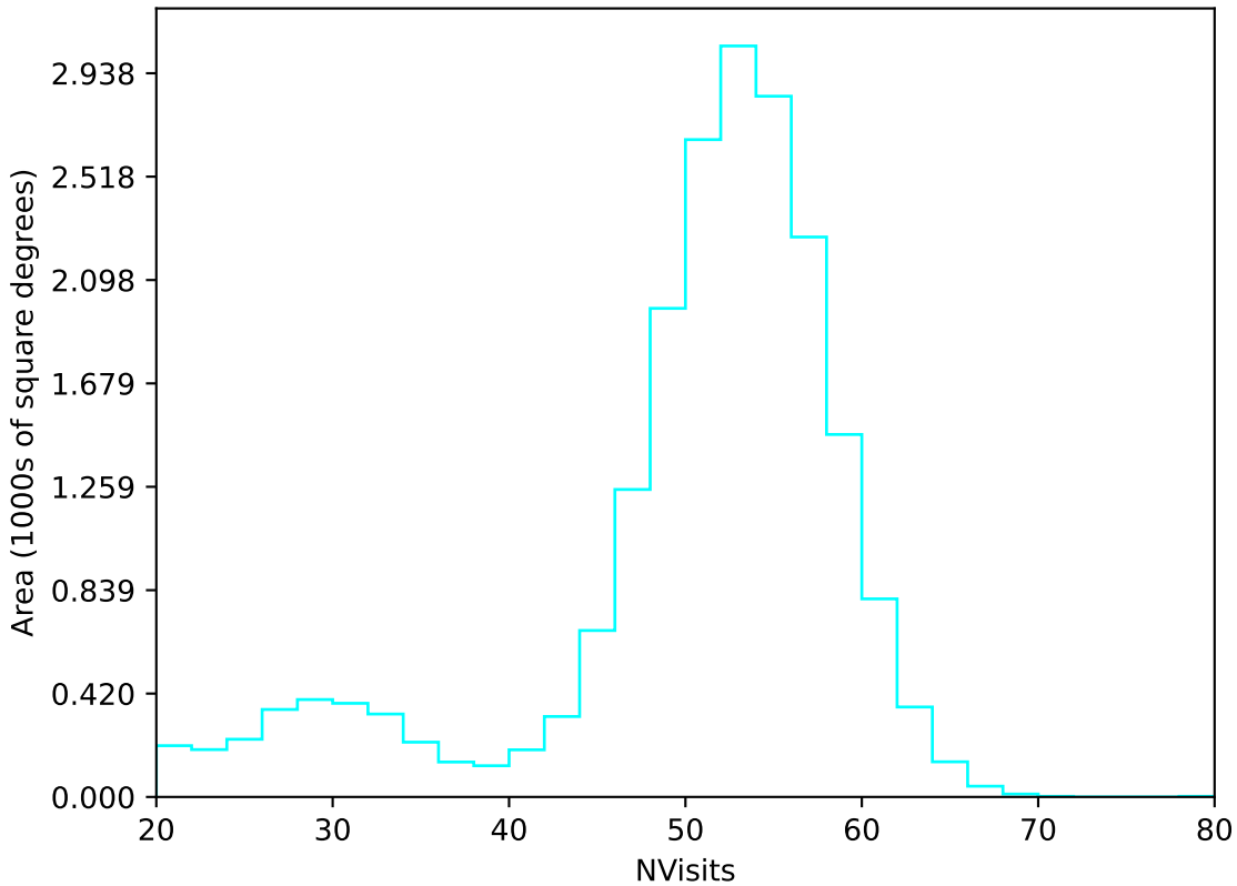
ddf_half_v3.4_10yrs All sky u band: NVisits
