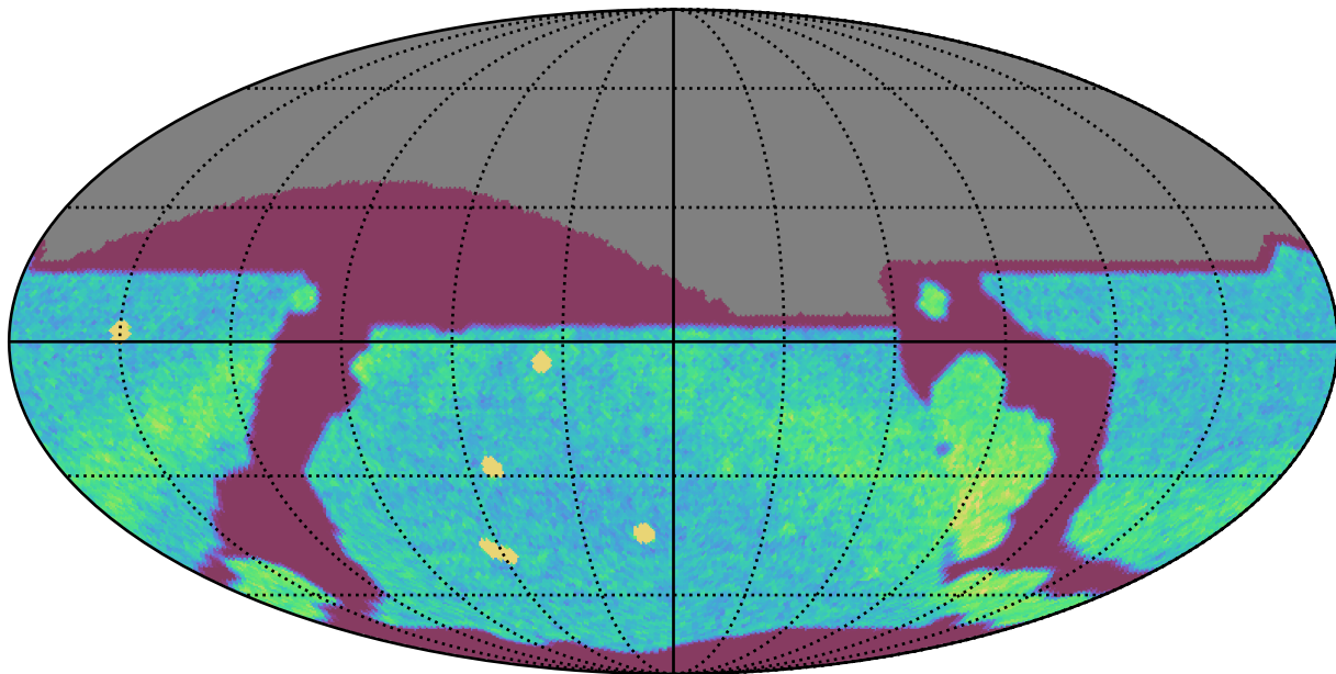
ddf_half_v3.4_10yrs All sky r band: NVisits
