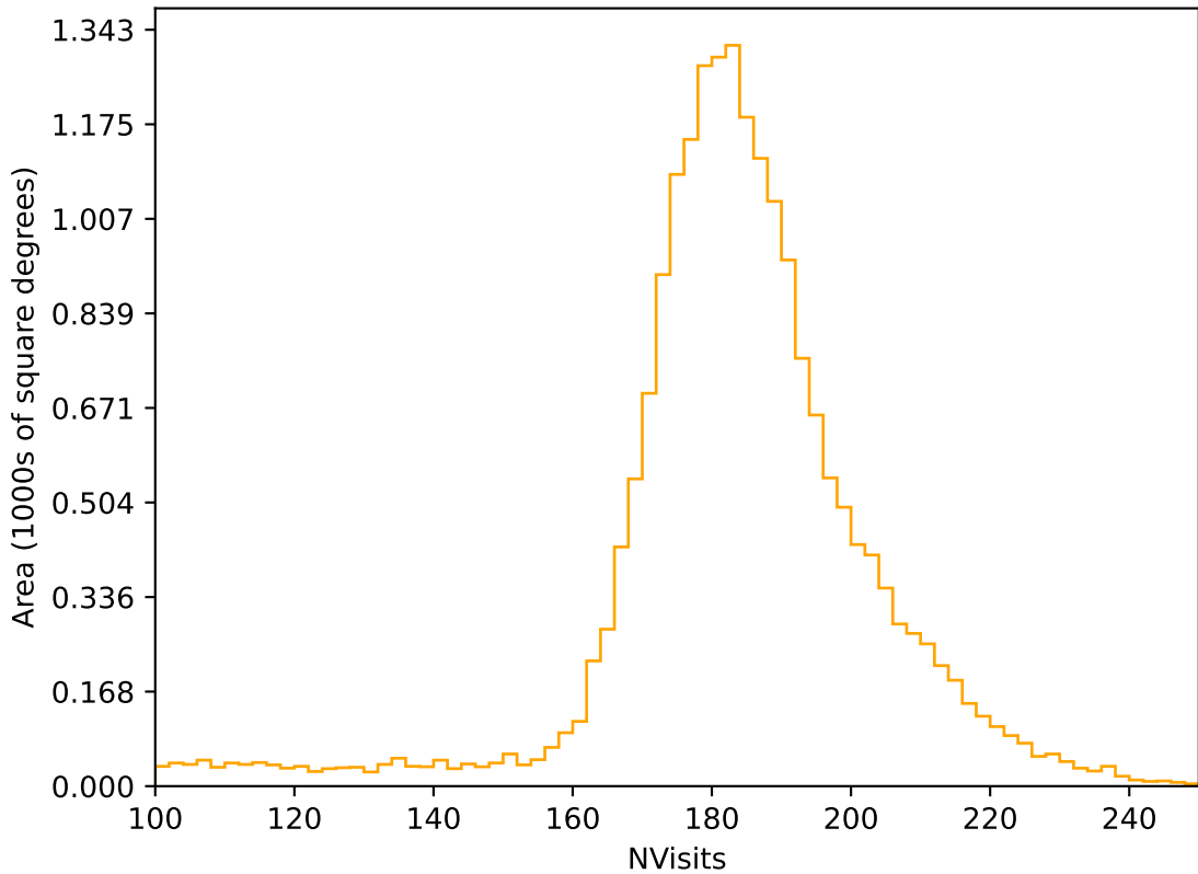
ddf_half_v3.4_10yrs All sky r band: NVisits
