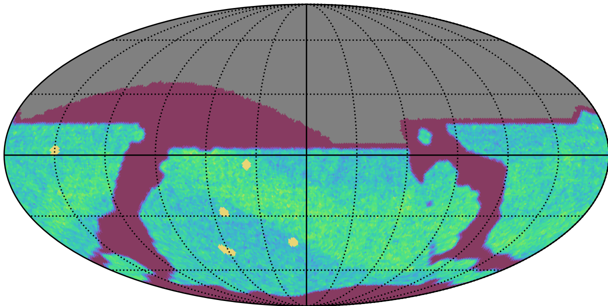
ddf_half_v3.4_10yrs All sky i band: NVisits
