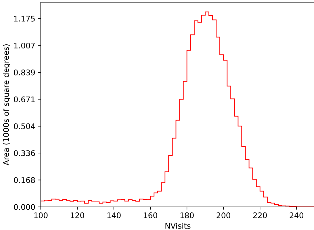
ddf_half_v3.4_10yrs All sky i band: NVisits
