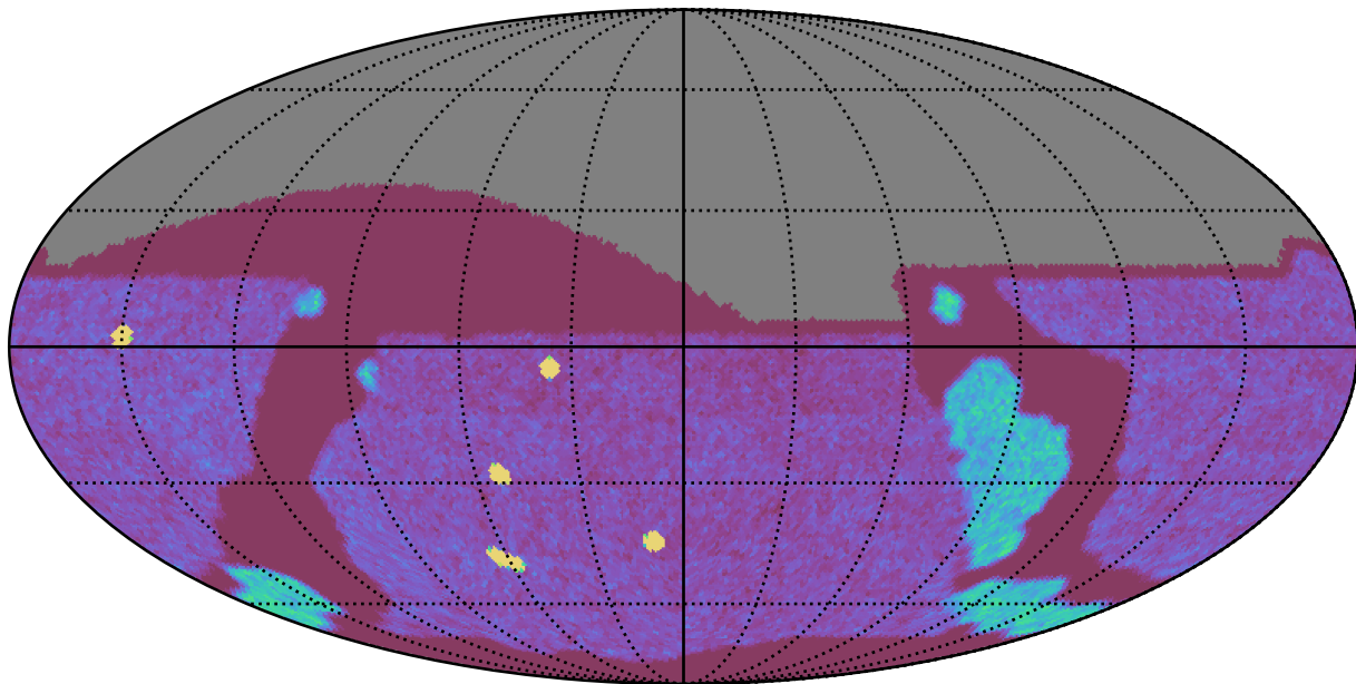
ddf_half_v3.4_10yrs All sky g band: NVisits
