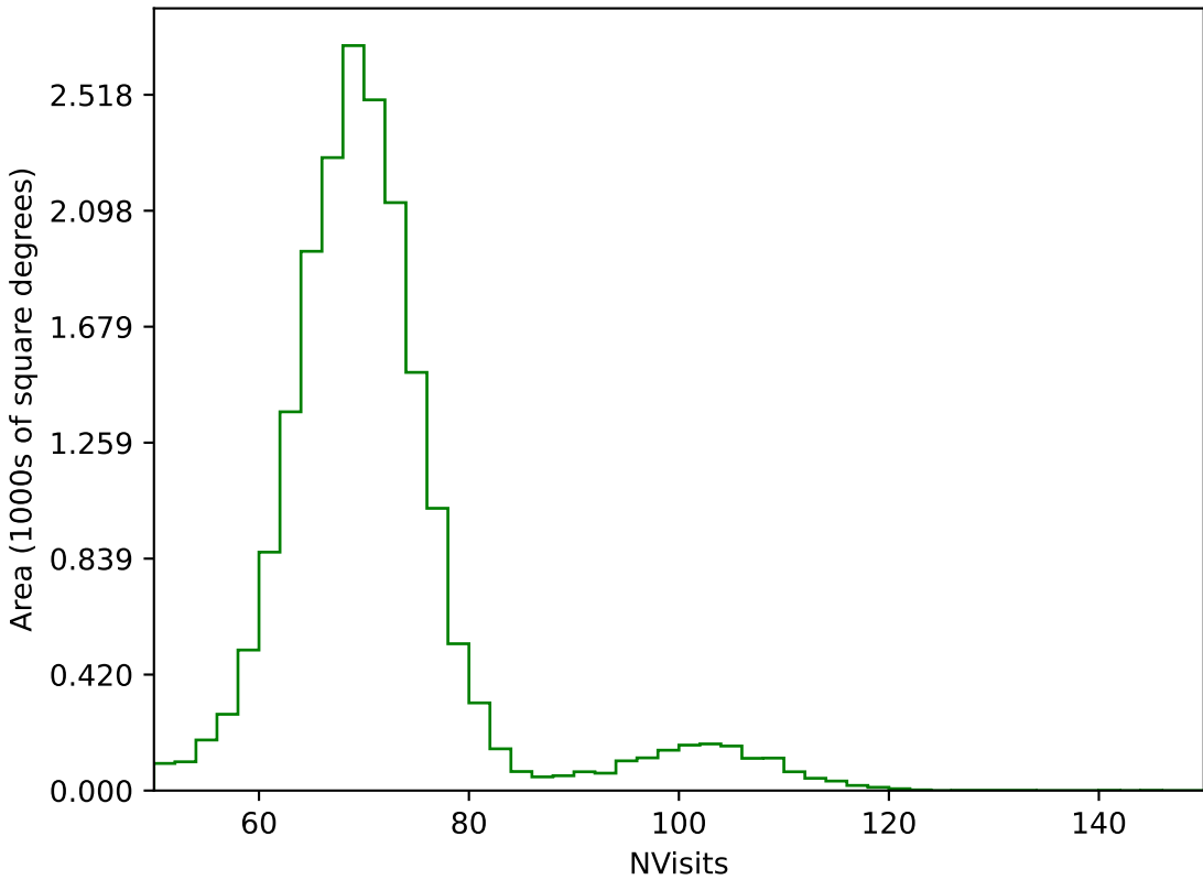
ddf_half_v3.4_10yrs All sky g band: NVisits
