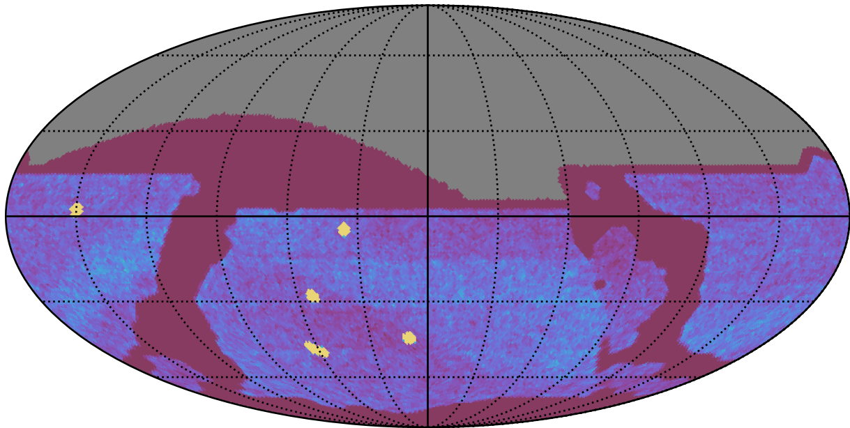
ddf_half_v3.4_10yrs All sky all bands: NVisits
