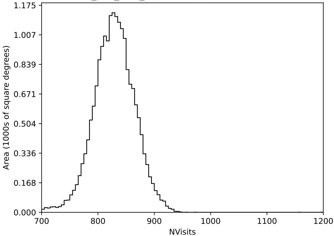
ddf_half_v3.4_10yrs All sky all bands: NVisits
