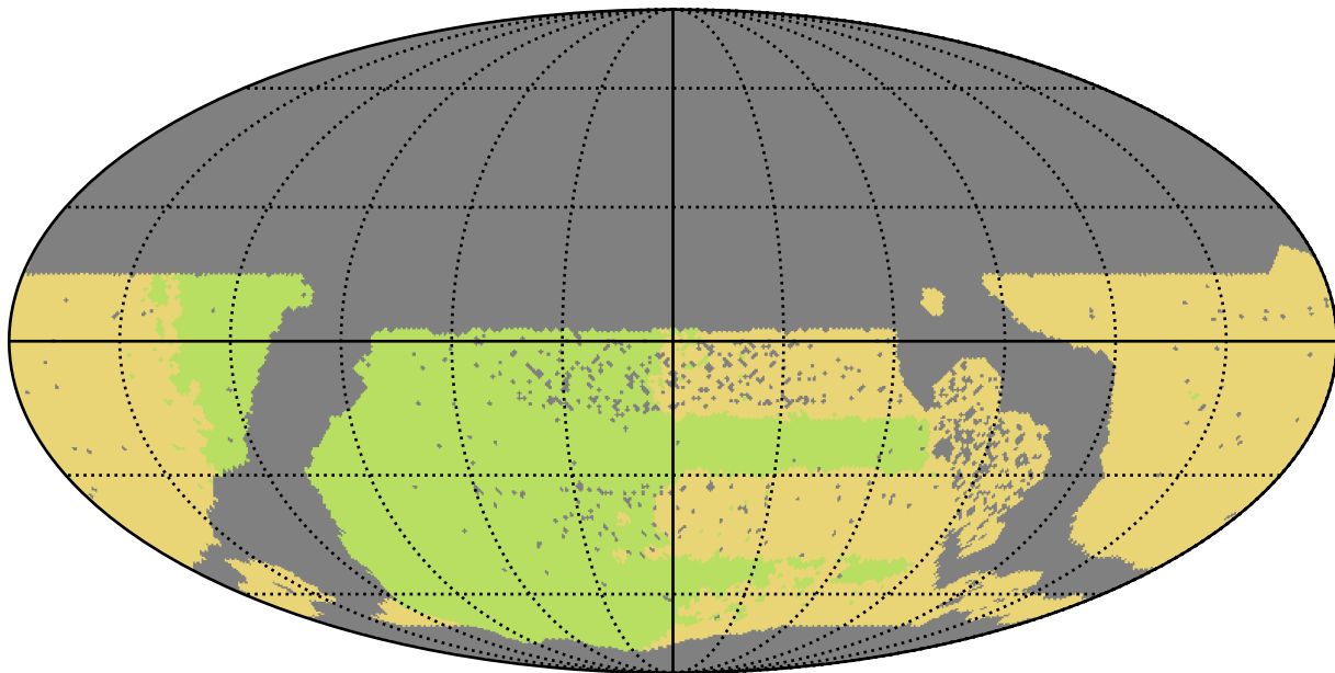
ddf_half_v3.4_10yrs WFD all bands: NSeasons
