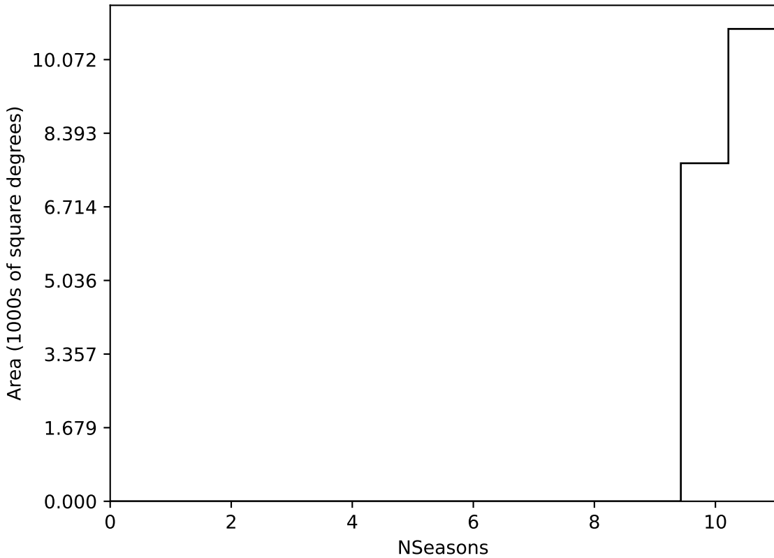
ddf_half_v3.4_10yrs WFD all bands: NSeasons
