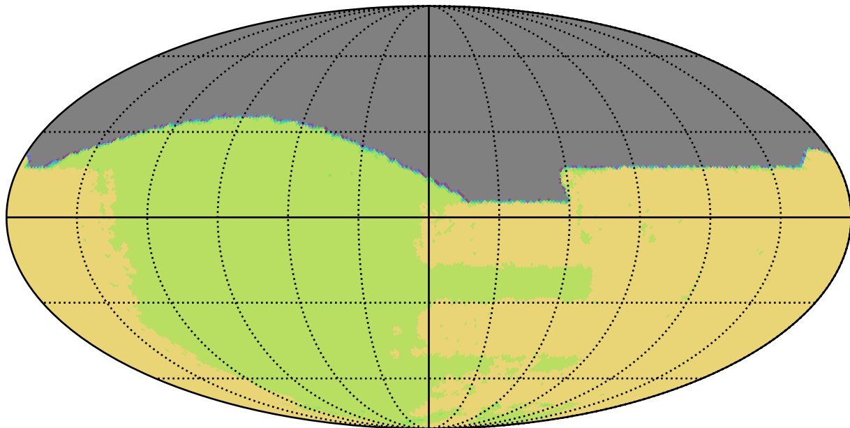
ddf_half_v3.4_10yrs All sky all bands: NSeasons
