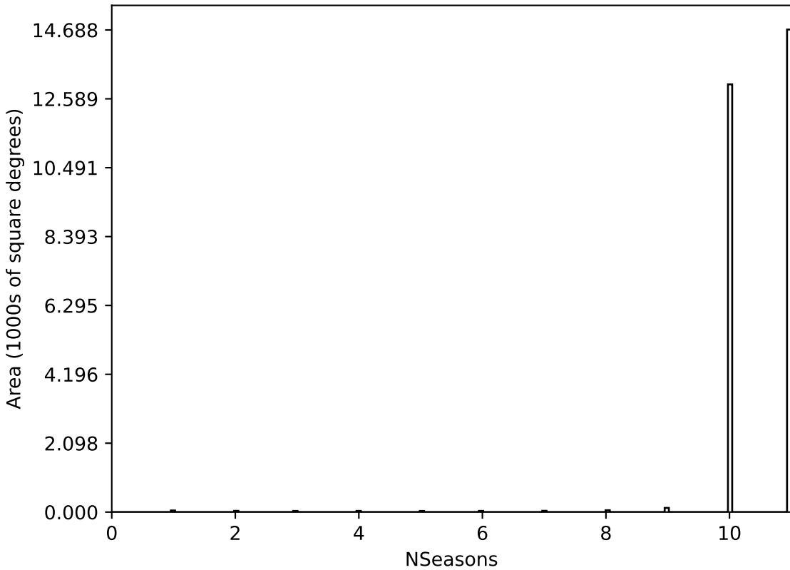
ddf_half_v3.4_10yrs All sky all bands: NSeasons
