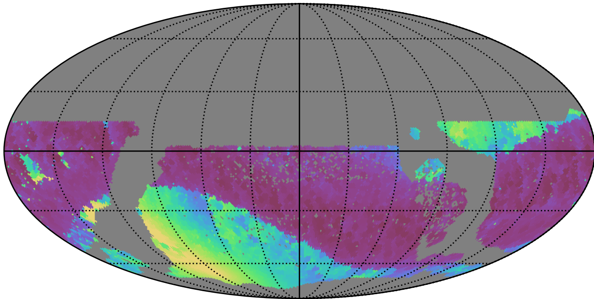
ddf_half_v3.4_10yrs WFD z band: Min solarElong
