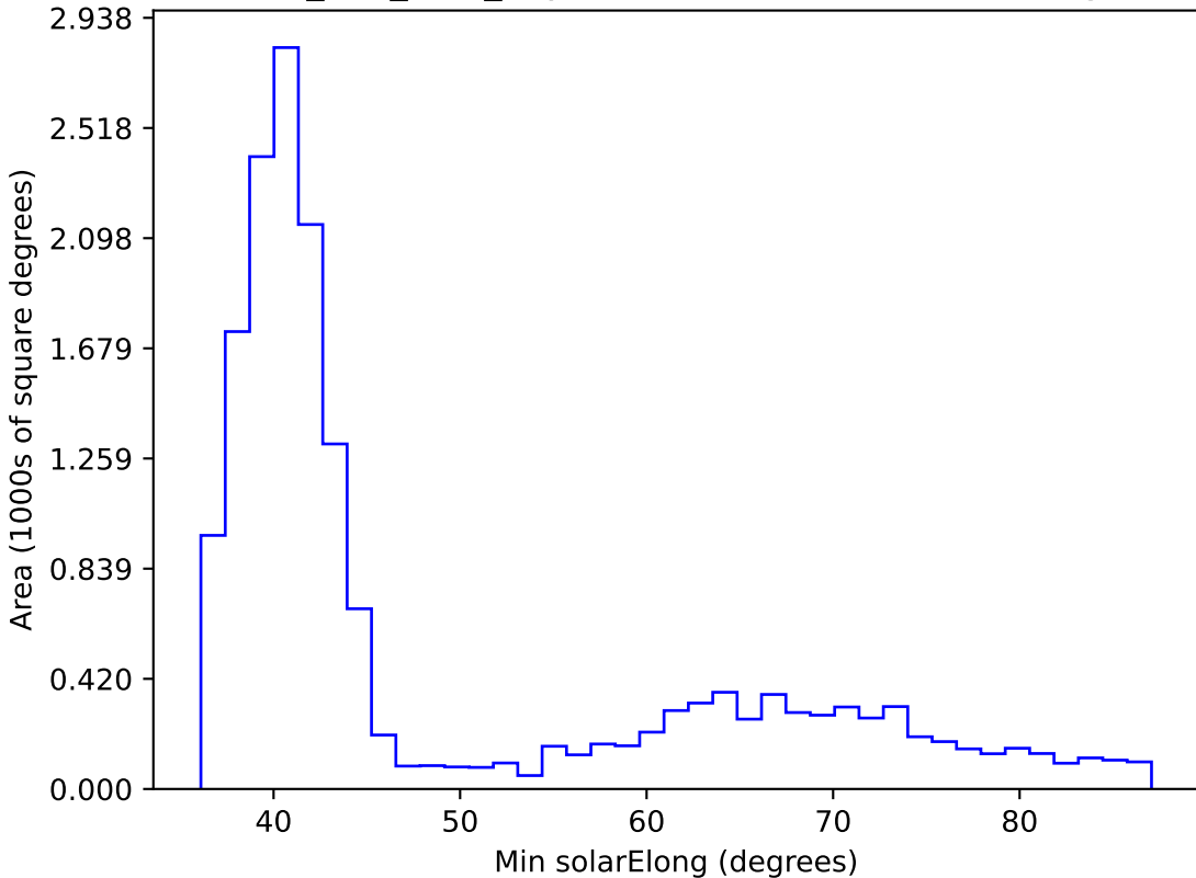
ddf_half_v3.4_10yrs WFD z band: Min solarElong
