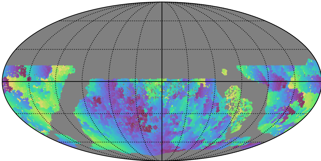
ddf_half_v3.4_10yrs WFD u band: Min solarElong
