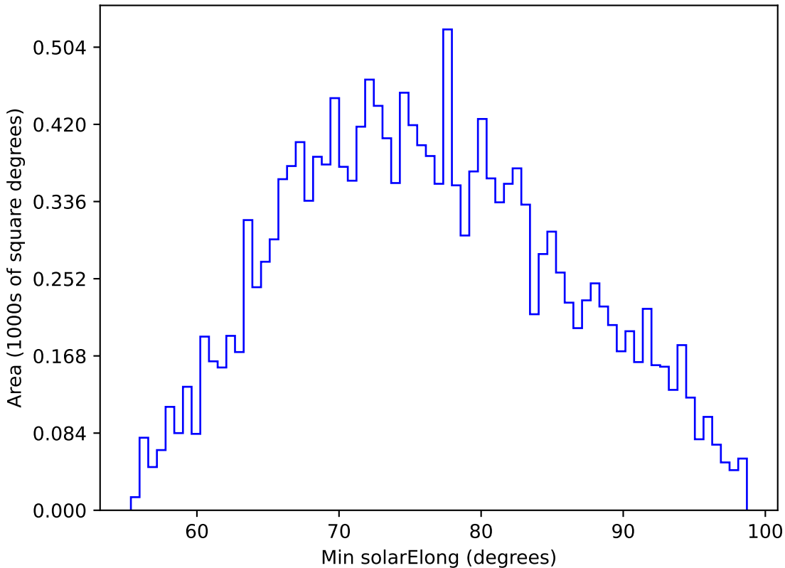
ddf_half_v3.4_10yrs WFD u band: Min solarElong
