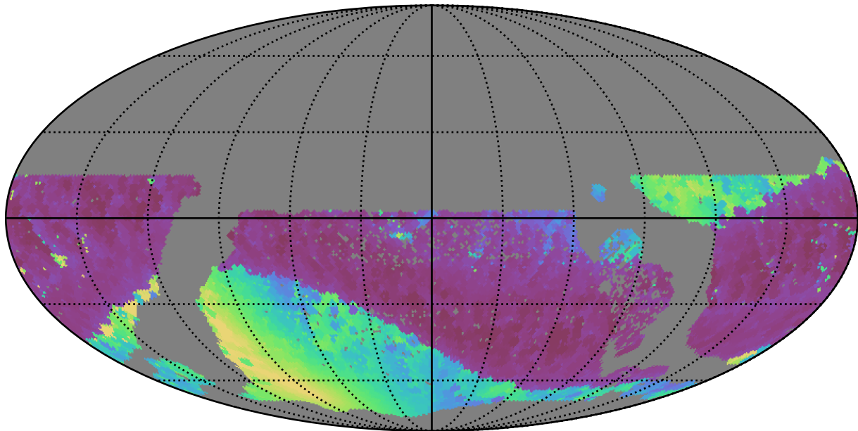
ddf_half_v3.4_10yrs WFD i band: Min solarElong
