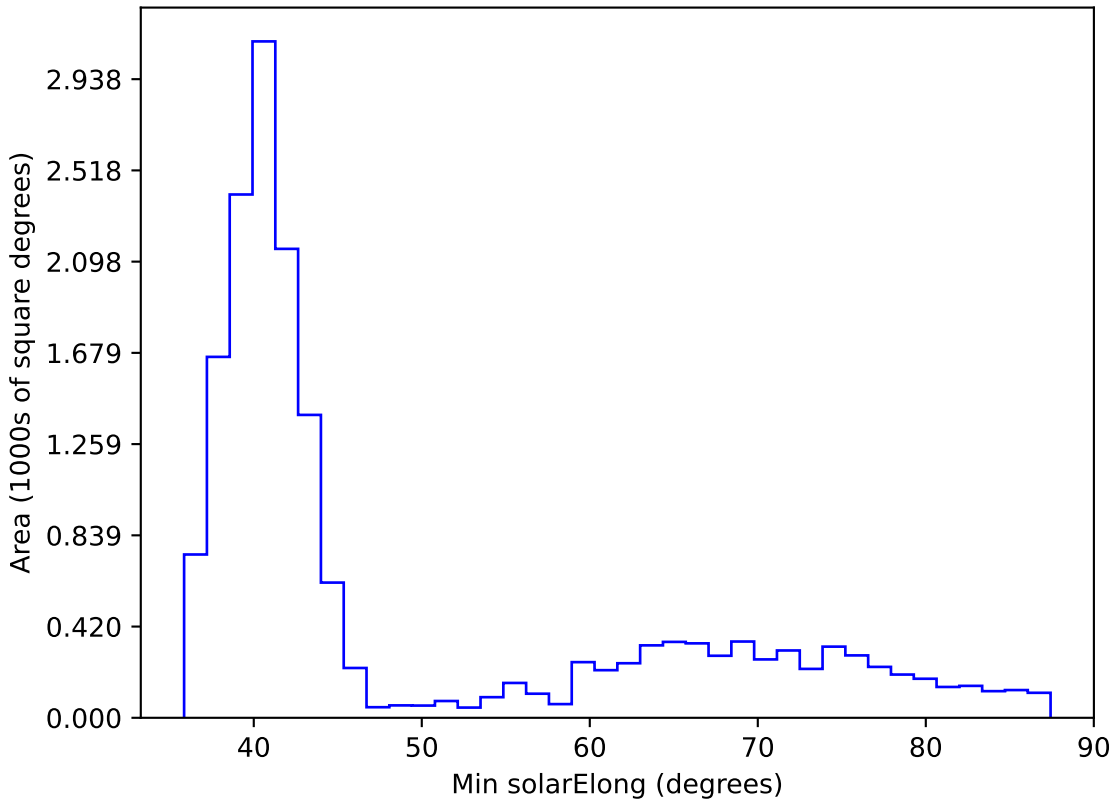
ddf_half_v3.4_10yrs WFD i band: Min solarElong
