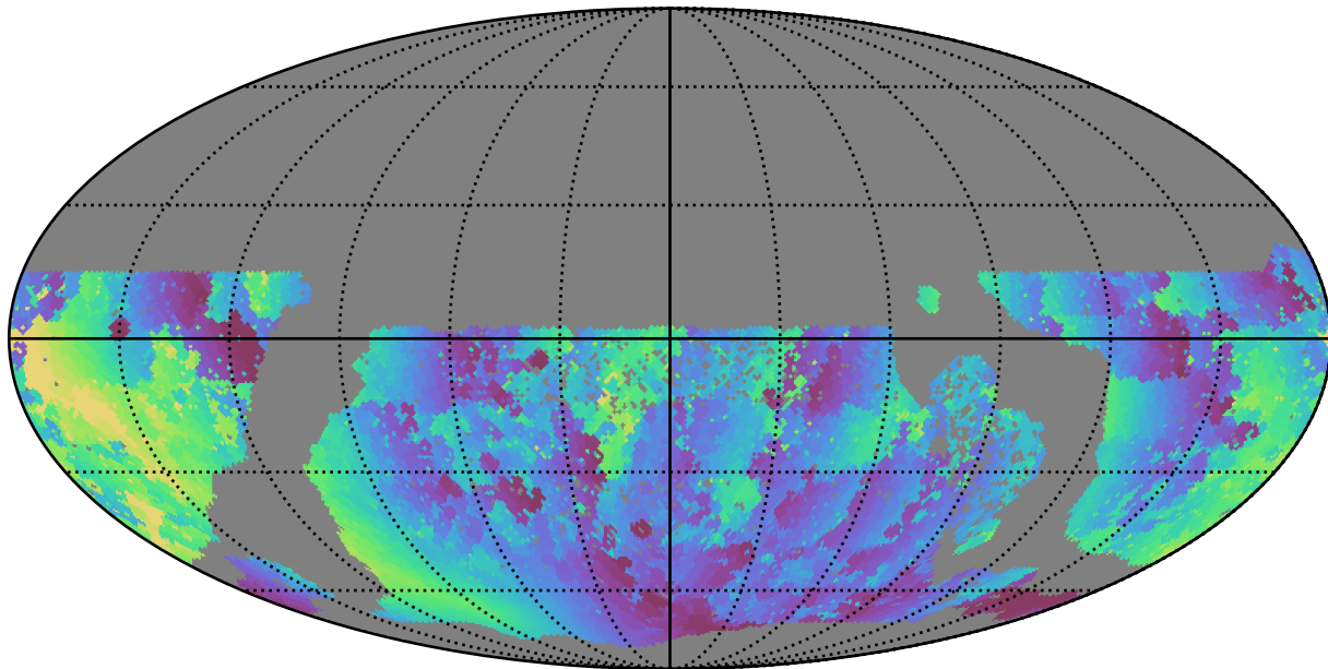
ddf_half_v3.4_10yrs WFD g band: Min solarElong
