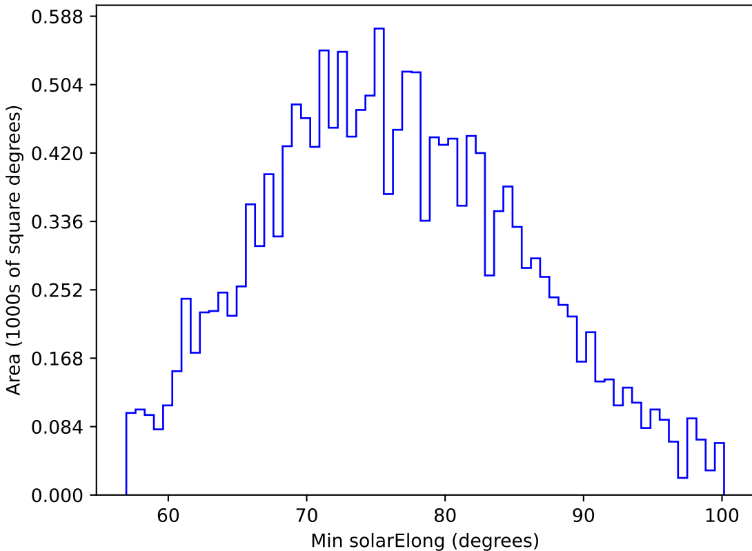
ddf_half_v3.4_10yrs WFD g band: Min solarElong
