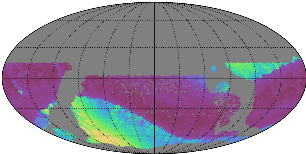
ddf_half_v3.4_10yrs WFD all bands: Min solarElong
