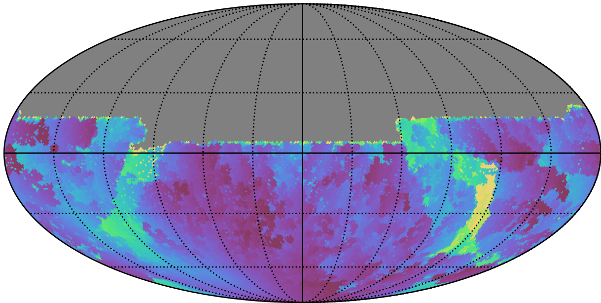
ddf_half_v3.4_10yrs All sky u band: Min solarElong
