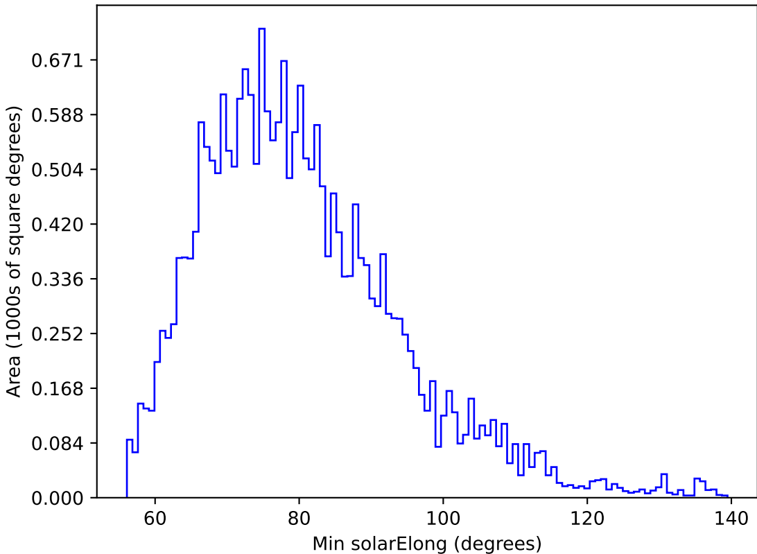
ddf_half_v3.4_10yrs All sky u band: Min solarElong
