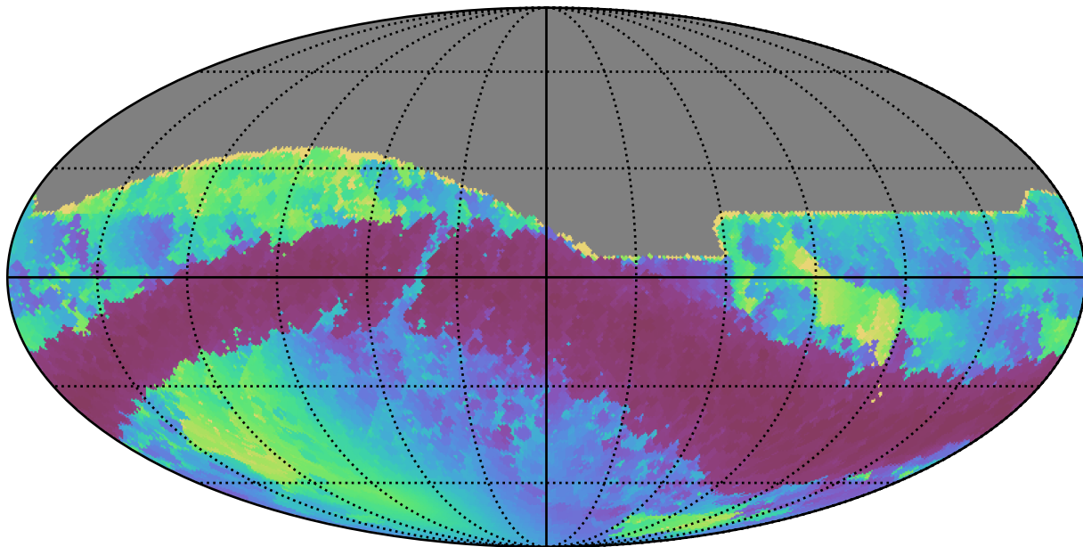
ddf_half_v3.4_10yrs All sky r band: Min solarElong
