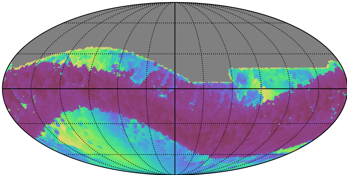
ddf_half_v3.4_10yrs All sky i band: Min solarElong
