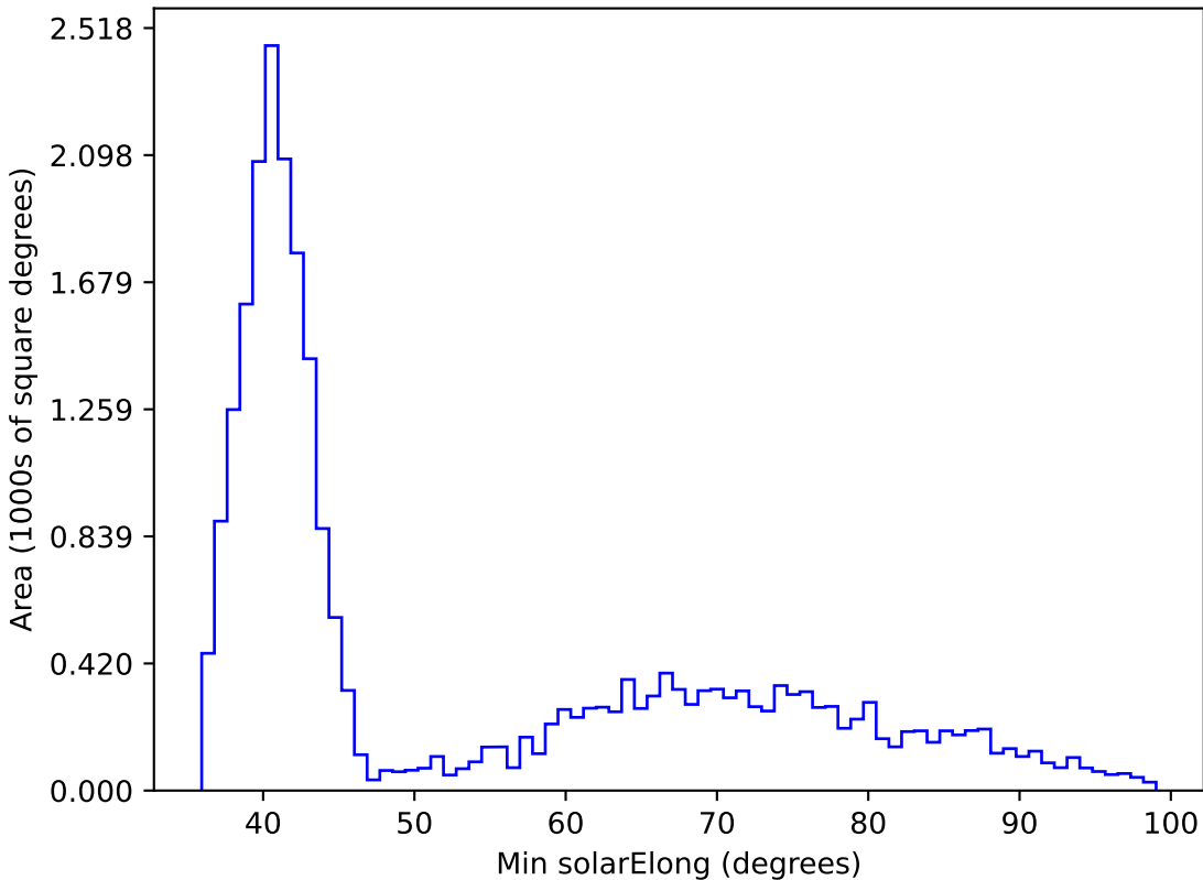
ddf_half_v3.4_10yrs All sky i band: Min solarElong
