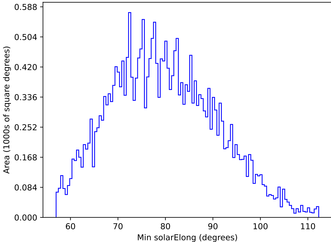
ddf_half_v3.4_10yrs All sky g band: Min solarElong
