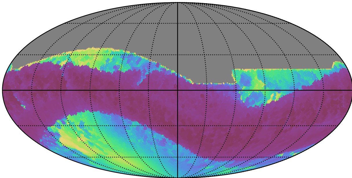
ddf_half_v3.4_10yrs All sky all bands: Min solarElong
