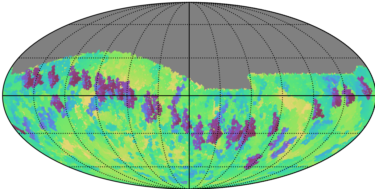
ddf_half_v3.4_10yrs Yr 1 z band: Min skyBrightness
