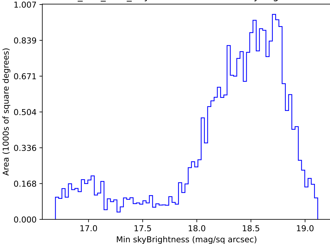
ddf_half_v3.4_10yrs Yr 1 z band: Min skyBrightness
