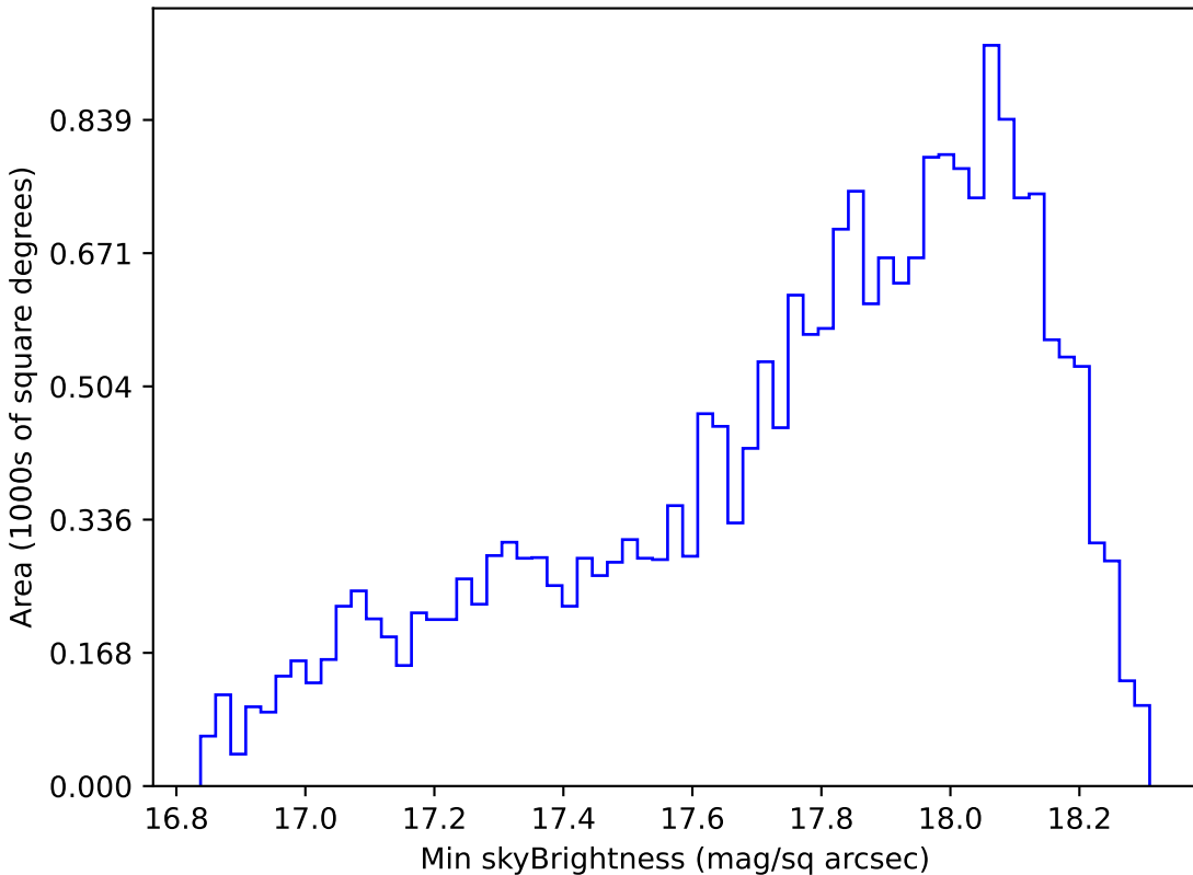
ddf_half_v3.4_10yrs Yr 1 y band: Min skyBrightness
