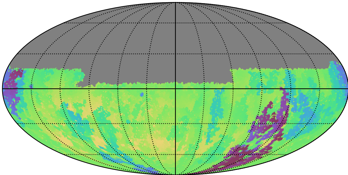
ddf_half_v3.4_10yrs Yr 1 u band: Min skyBrightness
