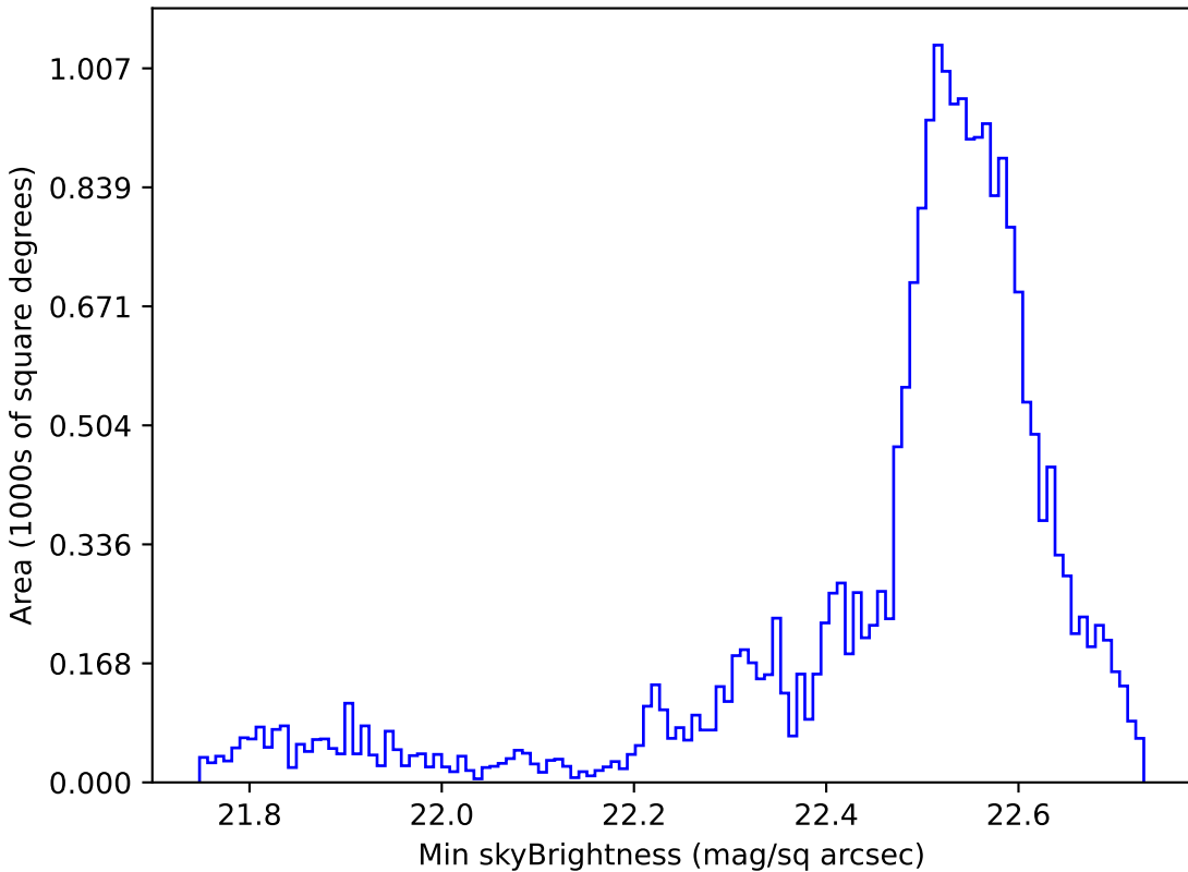
ddf_half_v3.4_10yrs Yr 1 u band: Min skyBrightness
