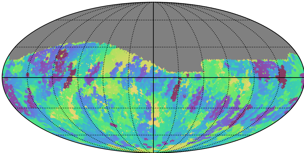
ddf_half_v3.4_10yrs Yr 1 r band: Min skyBrightness
