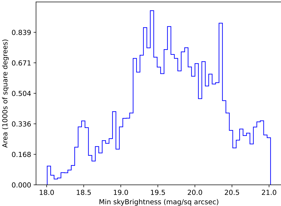
ddf_half_v3.4_10yrs Yr 1 r band: Min skyBrightness
