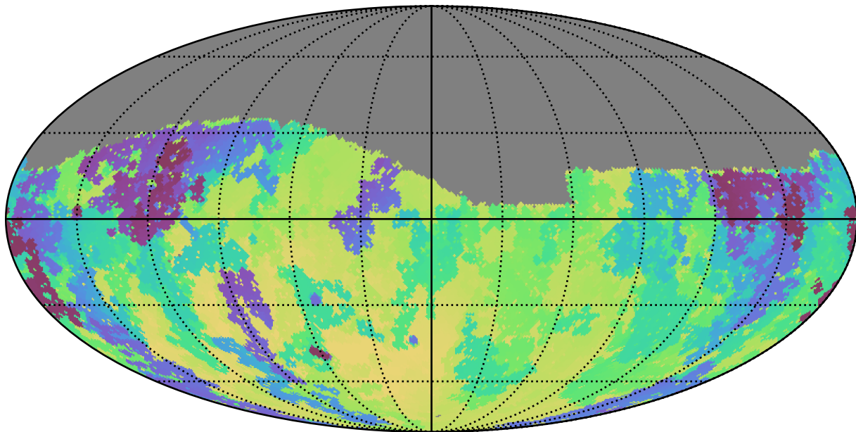
ddf_half_v3.4_10yrs Yr 1 g band: Min skyBrightness
