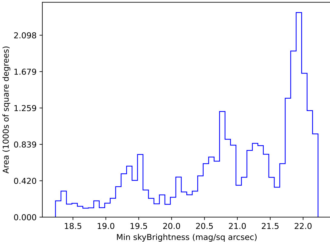
ddf_half_v3.4_10yrs Yr 1 g band: Min skyBrightness
