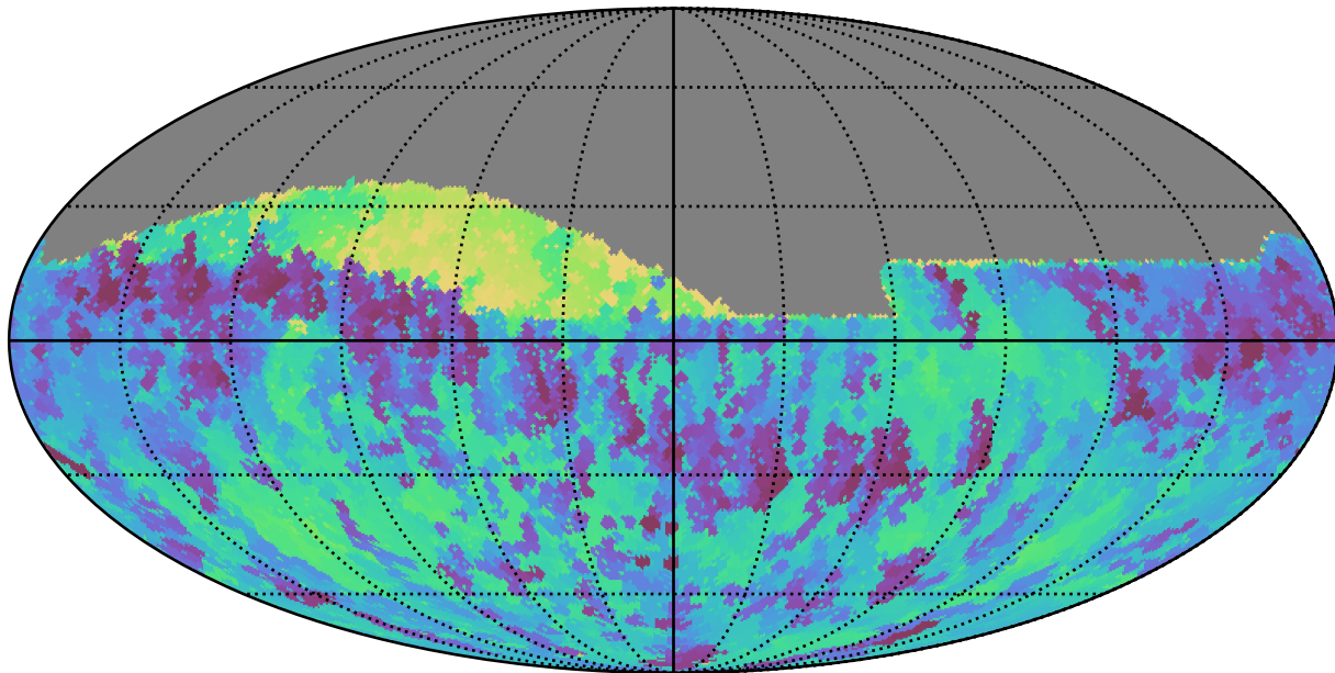
ddf_half_v3.4_10yrs Yr 1 all bands: Min skyBrightness
