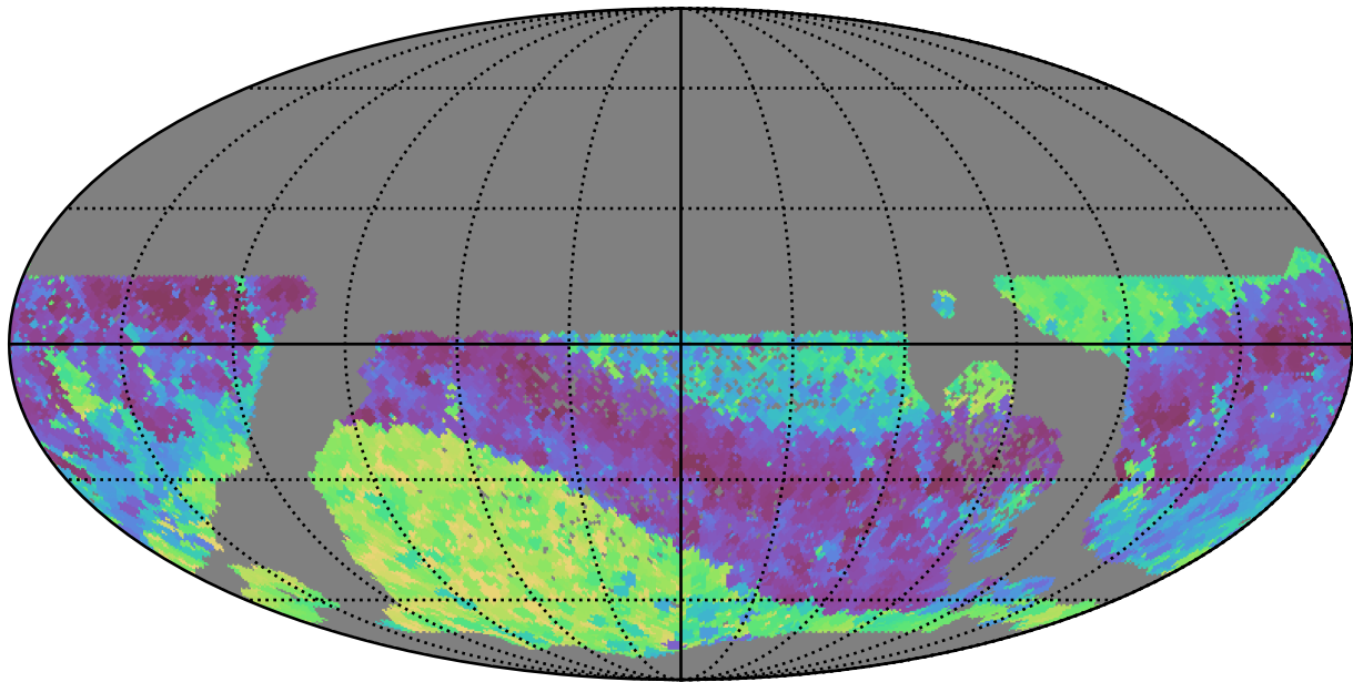
ddf_half_v3.4_10yrs WFD z band: Min skyBrightness
