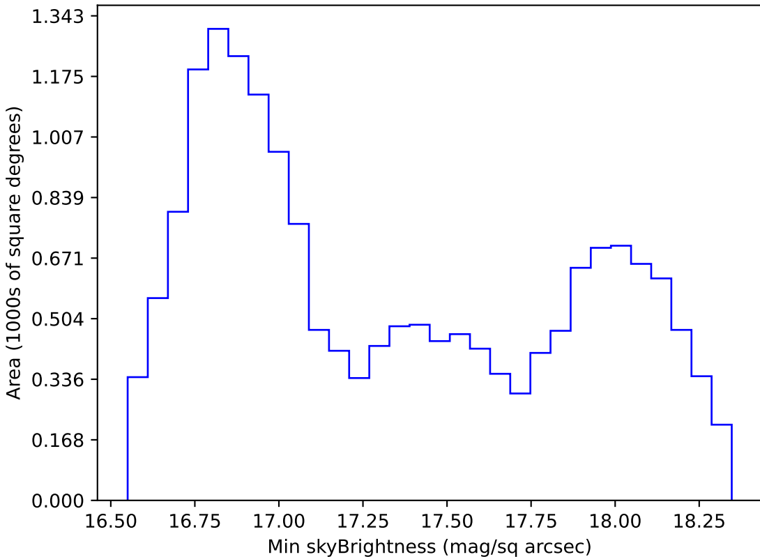
ddf_half_v3.4_10yrs WFD z band: Min skyBrightness
