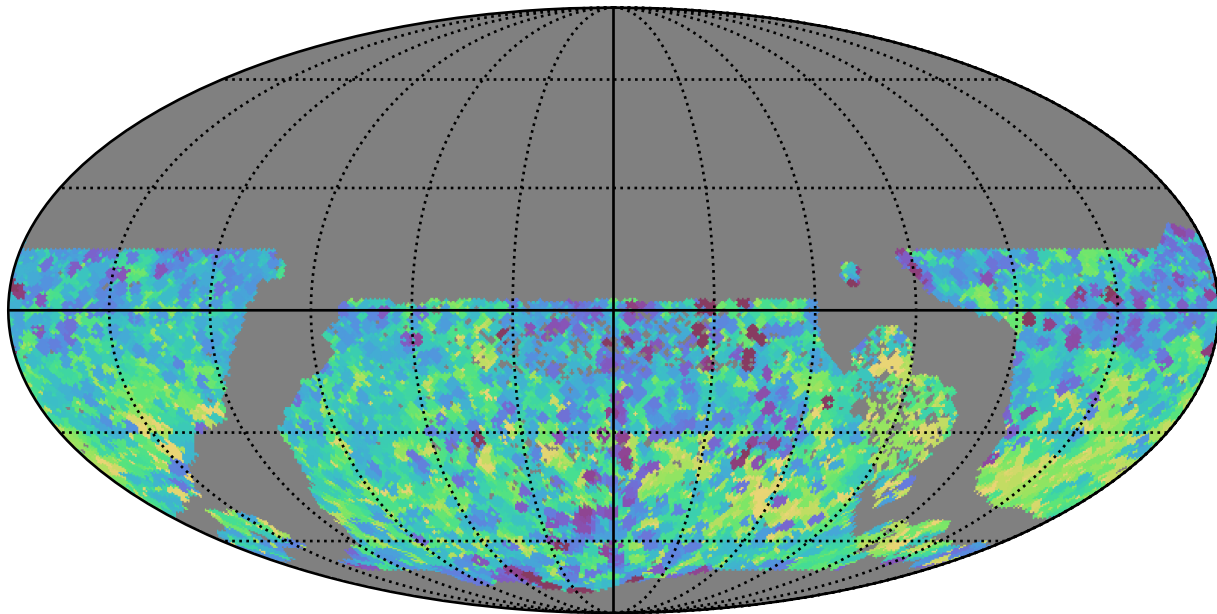
ddf_half_v3.4_10yrs WFD y band: Min skyBrightness
