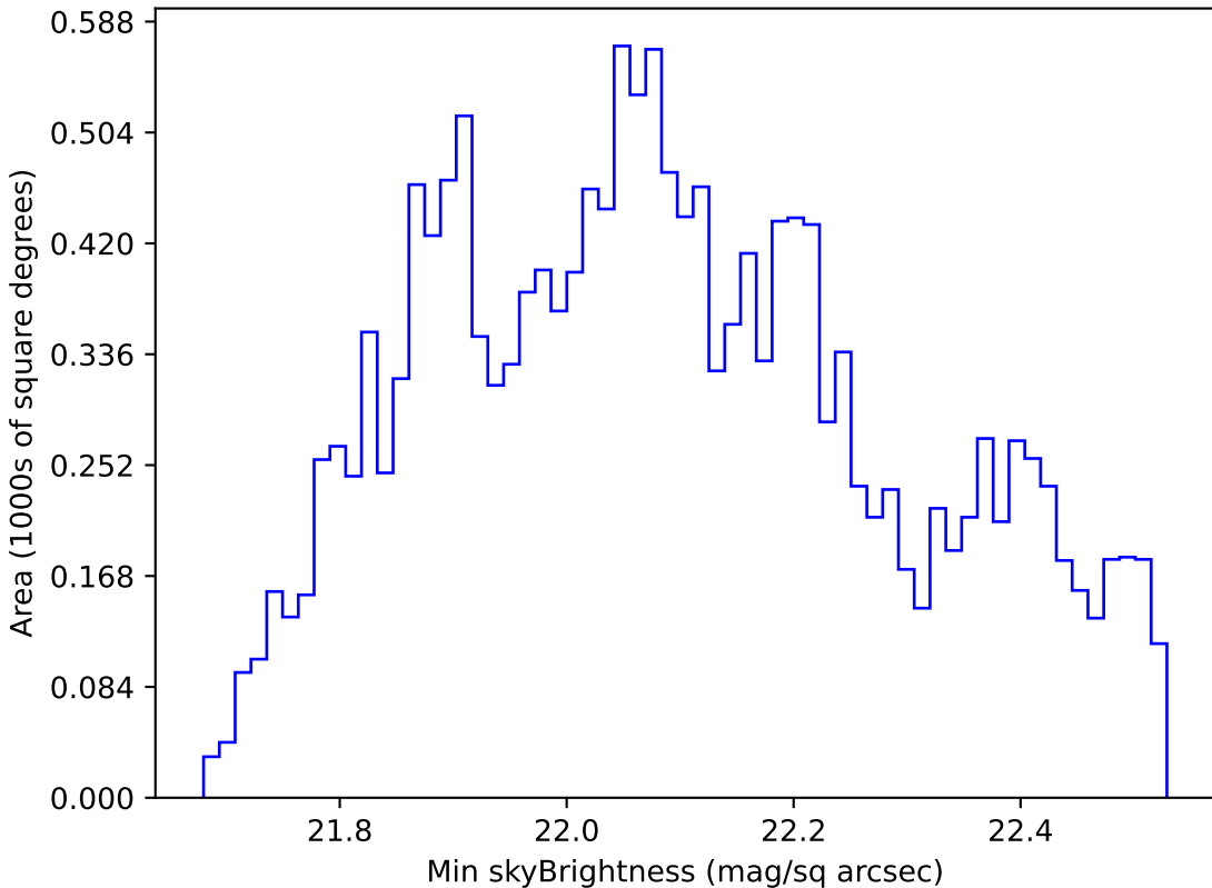
ddf_half_v3.4_10yrs WFD u band: Min skyBrightness
