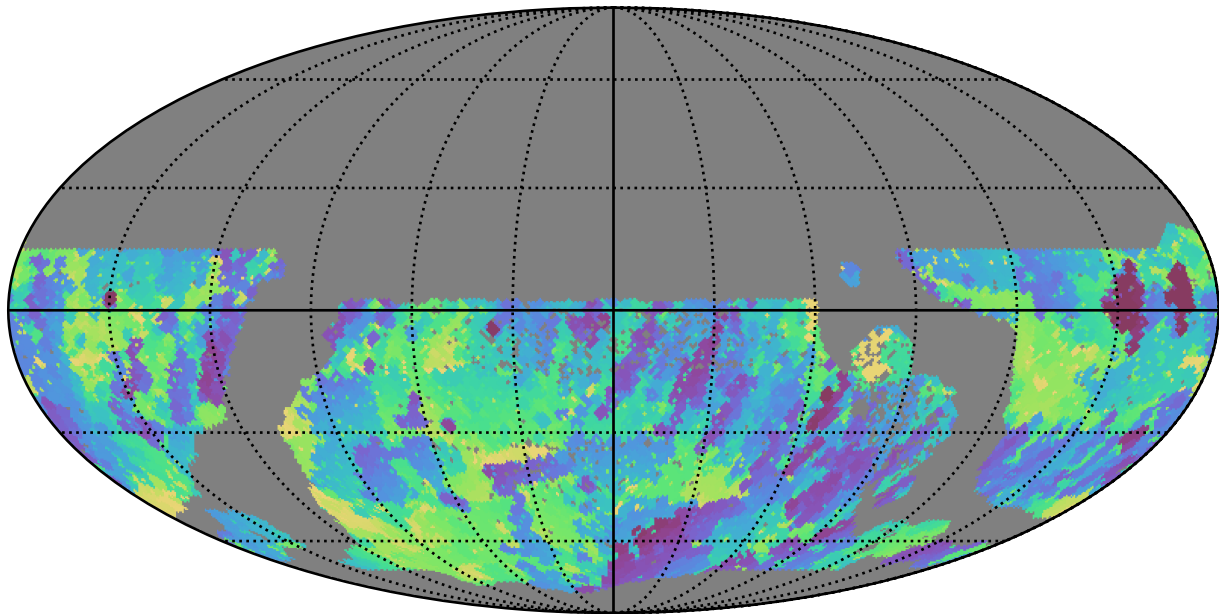
ddf_half_v3.4_10yrs WFD r band: Min skyBrightness
