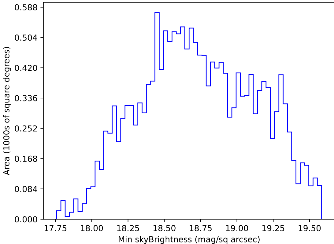
ddf_half_v3.4_10yrs WFD r band: Min skyBrightness
