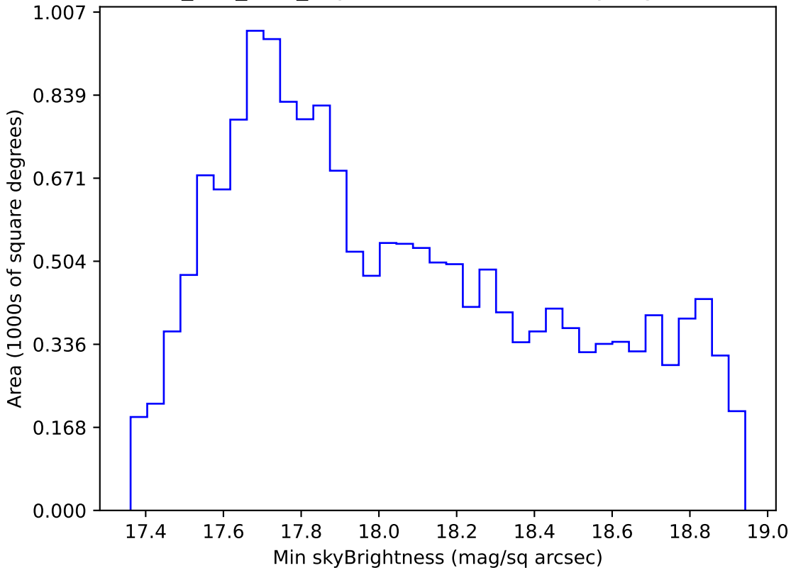
ddf_half_v3.4_10yrs WFD i band: Min skyBrightness
