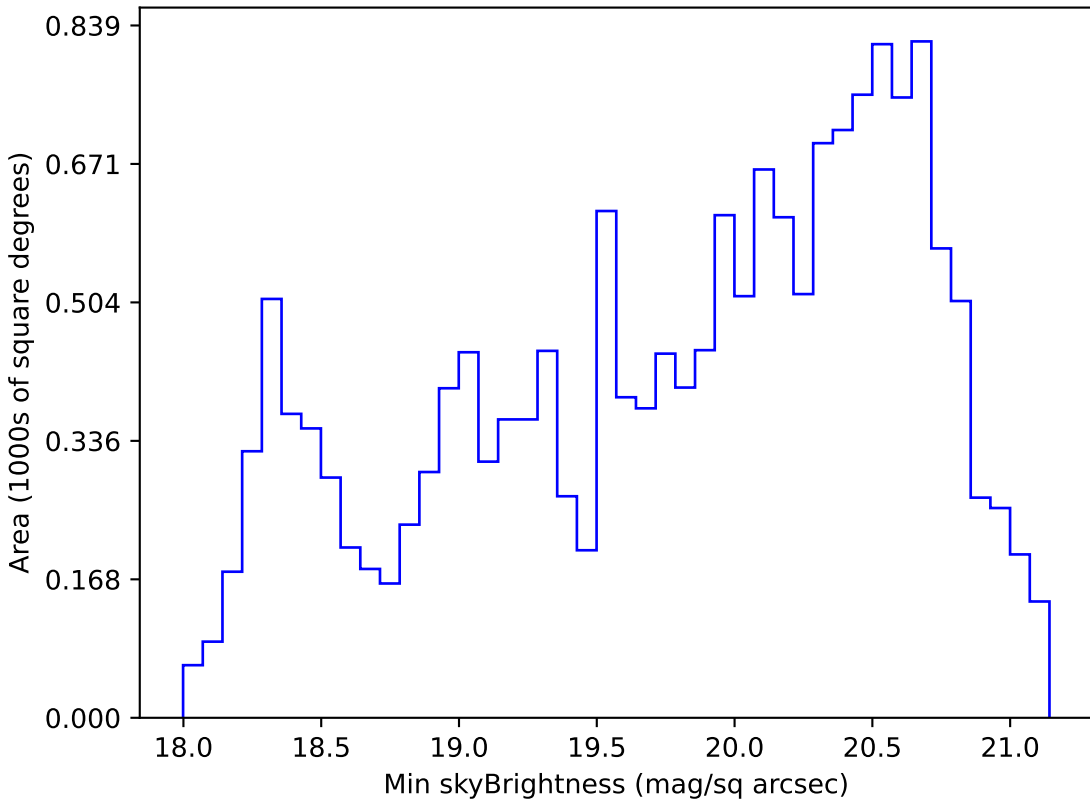
ddf_half_v3.4_10yrs WFD g band: Min skyBrightness
