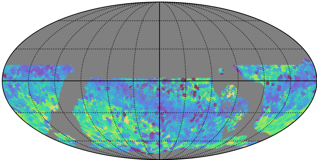
ddf_half_v3.4_10yrs WFD all bands: Min skyBrightness
