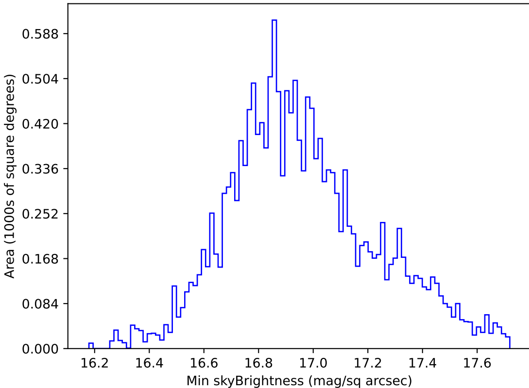
ddf_half_v3.4_10yrs WFD all bands: Min skyBrightness
